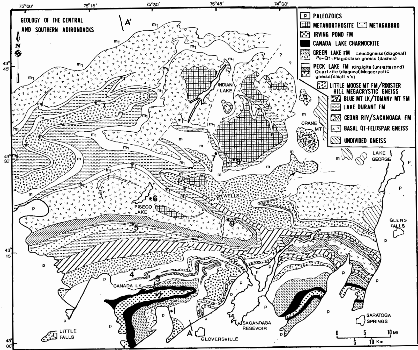
Fig. 2. Formational map and stop localities for the central and southern Adirondacks (from McLelland and Isachsen, 1980)
