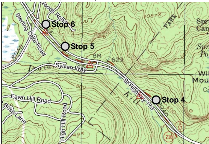
Figure 29. Topographic map showing the locations of Stops 4, 5 and 6 along Route 17A.
