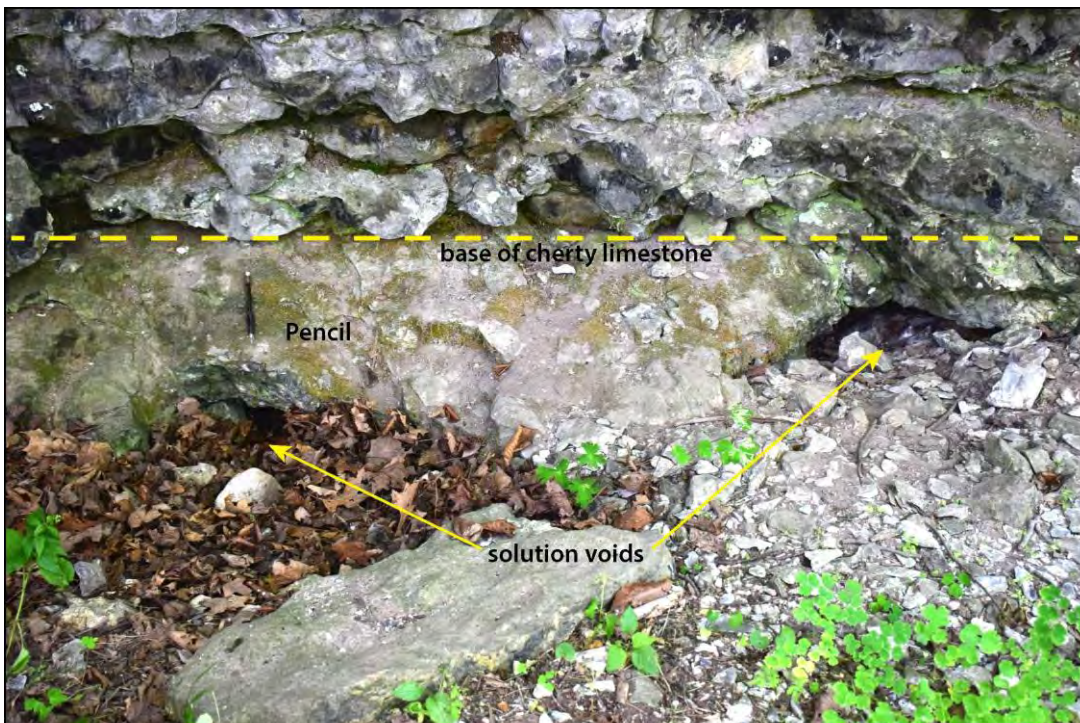
Figure 2-8. Two small solution voids in a limestone-rich bed beneath cherty limestone. Pencil for scale. The voids appear to have formed along a joint ( 068^{\circ} 83' SW) - bedding ( 009^{\circ} 13' NW) intersection. Photo by Don Monteverde.
