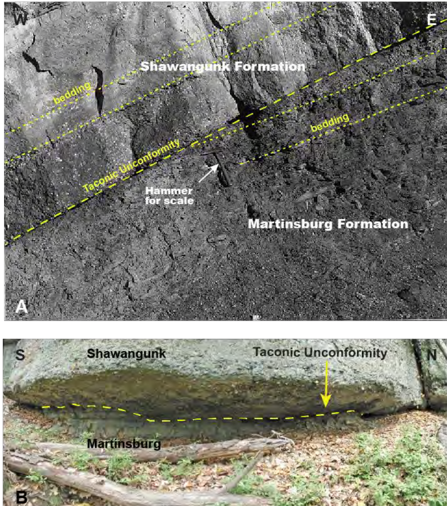
Figure 3 - Exposure of the Taconic unconformity. A) exposure looking north taken during construction of Interstate Route 84 in New York by Epstein. Note slight angular divergence between the Shawangunk and Martinsburg sediments. B) exposure looking west taken south of Sunrise Mountain in Stokes State Forest, New Jersey by Monteverde. Surface shows evidence of minor slip.
