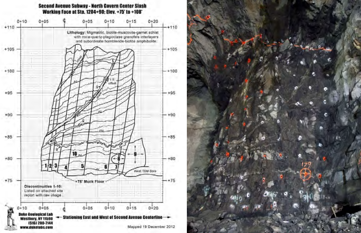
Figure 13 - Isoclinal recumbent folds of early SE-dipping foliation in Hartland formation (OCh) outlined by granitoid sills (g) with gently inclined penetrative foliation. Recrystallization during folding and shearing produces penetrative mica foliation (Feature 10.) that has formed parallel to compositional layering. Gently inclined foliation joints are prominent discontinuities ( J_1 ) and have formed parallel to the foliation and parallel compositional layering. These are intersected by steep NE-trending ( J_2 ) and NW-trending ( J_3 ) joints and faults producing overbreak seen at top of image. (Digital image taken 19 December 2012.)
