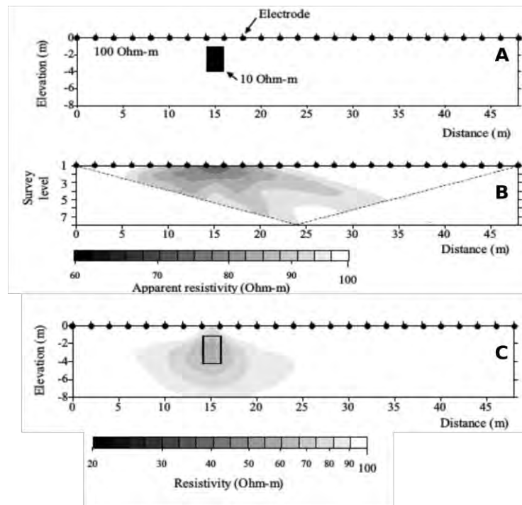
Figure 5: Example of electrical data acquisition and processing. A) the true model of subsurface, B) the pseudo-section of the acquired data, and C) the inverted image of 'real' resistivity distribution. (adapted from [Binley and Kemna, 2005])
