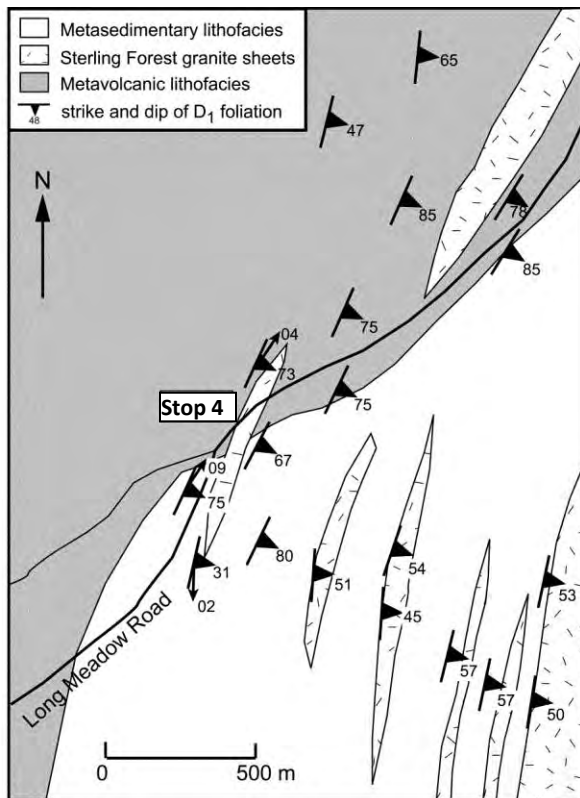
Figure 14. Geologic map showing the location of Stop 4.
