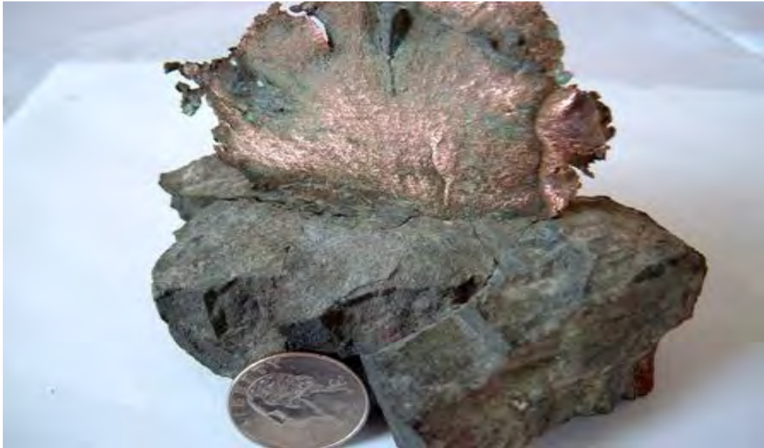
Figure 3. Sheet of native copper in basalt joint sampled at the Chimney Rock trap-rock quarry, New Jersey
