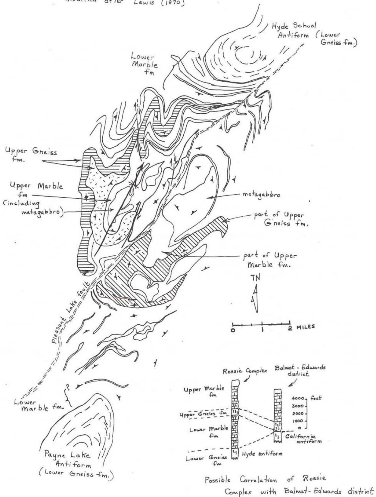
FIG. 8. Geology of the Rossie Complex (SW of Hyde alaskite body)
