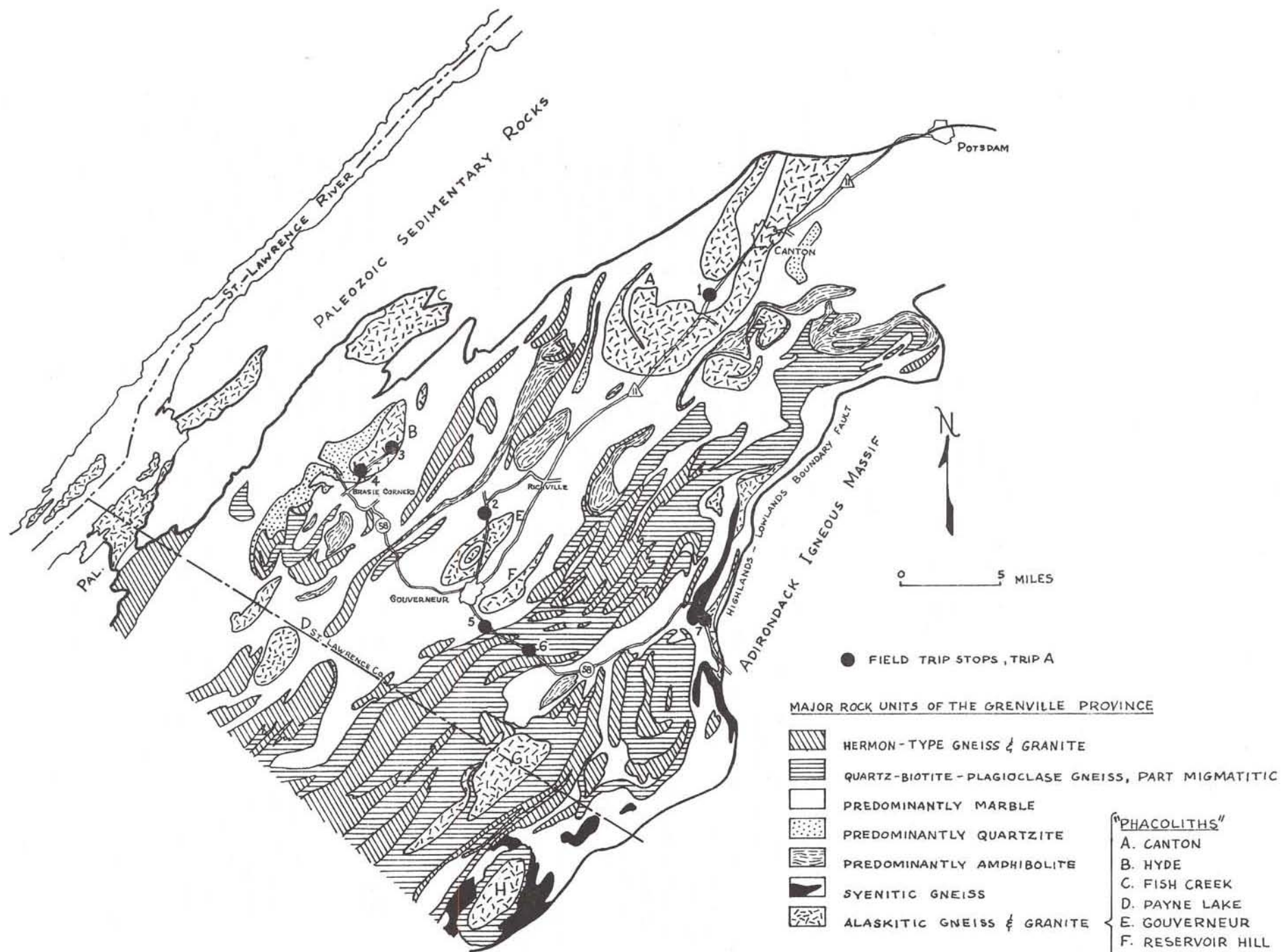
FIG.2. GENERALIZED GEOLOGIC MAP OF NORTHWEST ADIRONDACKS (AFTER BROUGHTON et al. , 1962) (PALEOZOIC OUTLIERS OMITTED)
