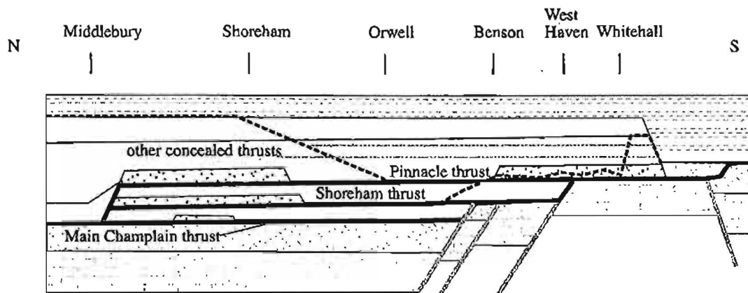
Figure 10. Along-strike cross-section across figure 4 demonstrating the change in stratigraphic level of thrusts across transverse cross-faults. The Mettawee fault is drawn with a dashed line, and the geology now cut-out by the fault is interpreted.
