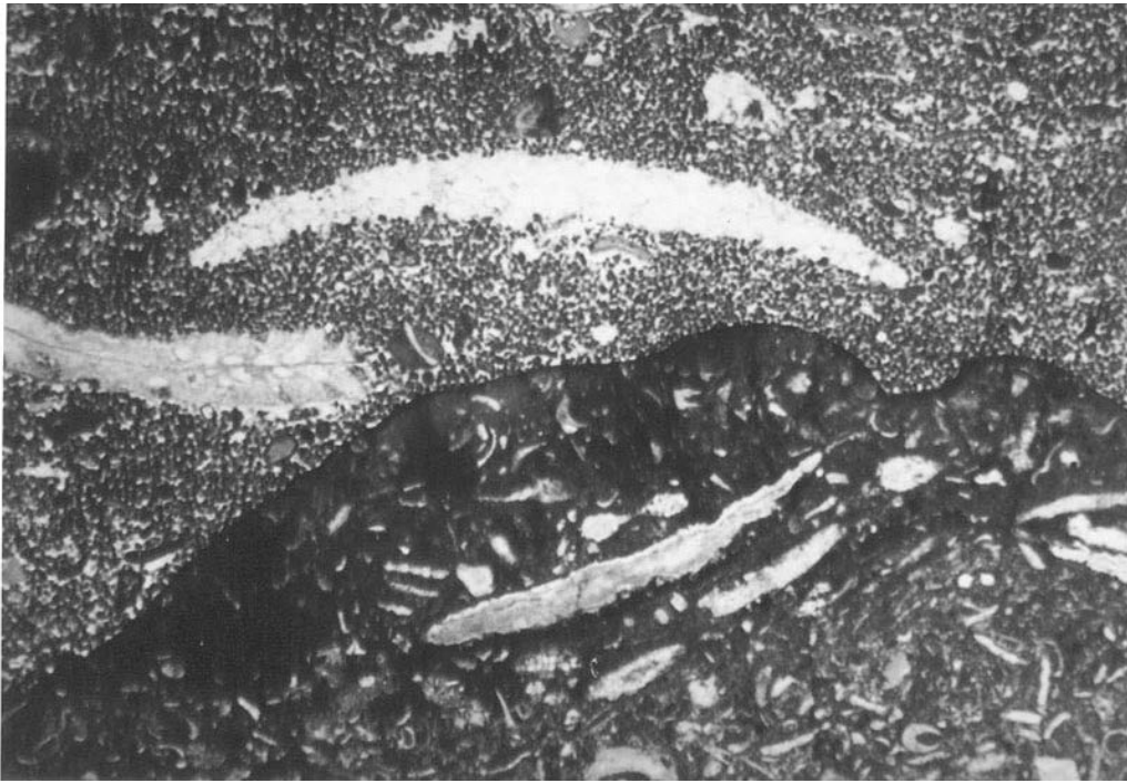
Figure 13. Thin section photomicrograph of a firmground; field of view is 1.5cm
