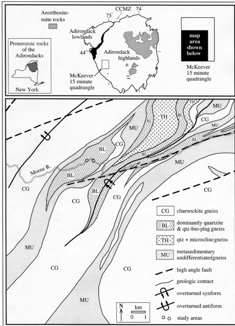
Fig. 10. - Map showing location of prismatic-bearing metapelites and quartzites (open circles on Moose River) and surrounding bedrock geology. Stop 6 is the easternmost open circle. Geologic map units, structures, and relations illustrated are from Whitney et al. (2002). Taken from Darling et al. (2004). Bio—biotite; CCMZ—Carthage-Colton mylonite zone; pl—plagioclase; qtz—quartz.
