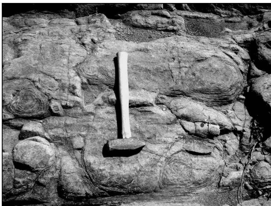
Figure 4. – Vertical view onto surface of Ordovician–age, spheroidal weathering preserved in middle Proterozoic felsic gneiss just below the Knox unconformity at Roaring Brook (Stop 3). Hammer for scale.
